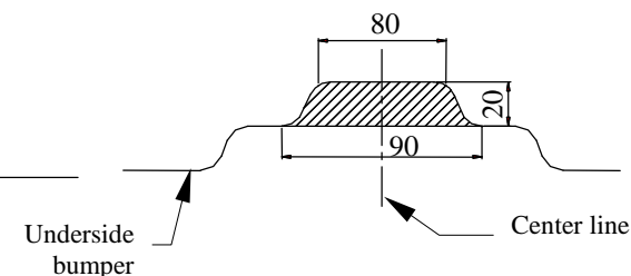
Fig. 3 Bumper cut out Mazda Tribute
